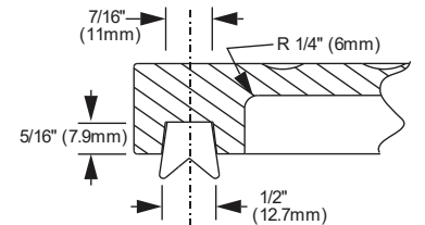
GASKET GROOVE, SECTION B:B
