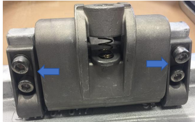
Figures 2a & 2b – Hinge Removal and Installation
